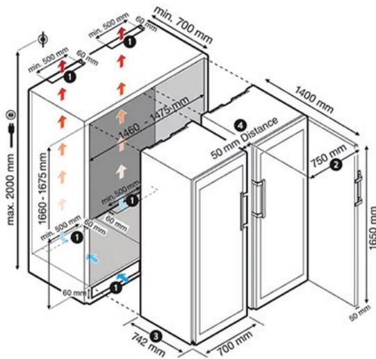
Side-by-Side Installation
